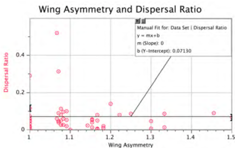
Figure 9 Effect of Asymmetry on Dispersal Ratio.
