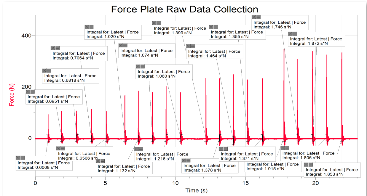
Figure 4 Data from the force plate is shown. The integral of each of the hits were calculated to find the impulse of each hit.
