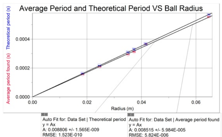
Figure 4 The periods of sound produced by the spheres and the theoretical periods as predicted by spherical harmonics, as compared to the radii of the balls, for the first resonance mode.
