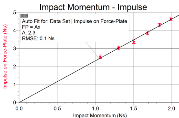
Figure 4: The proportional fit of the graph for impact momentum against impulse.
