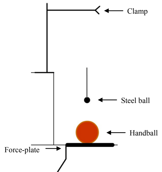
Figure 3: The experimental setup.
