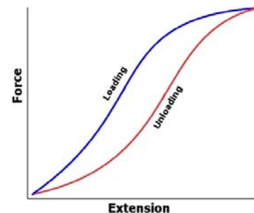
Figure 1 Idealized graph of elastic hysteresis for rubber. [3]
