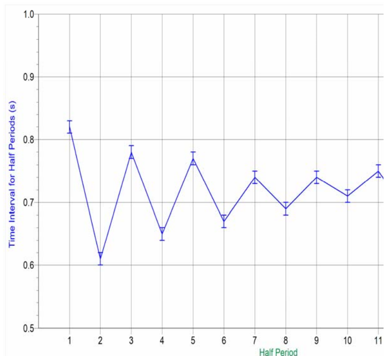
Fig 8: Time Interval between Half Periods. The difference in half periods reduces with amplitude, while the whole period remains constant.
