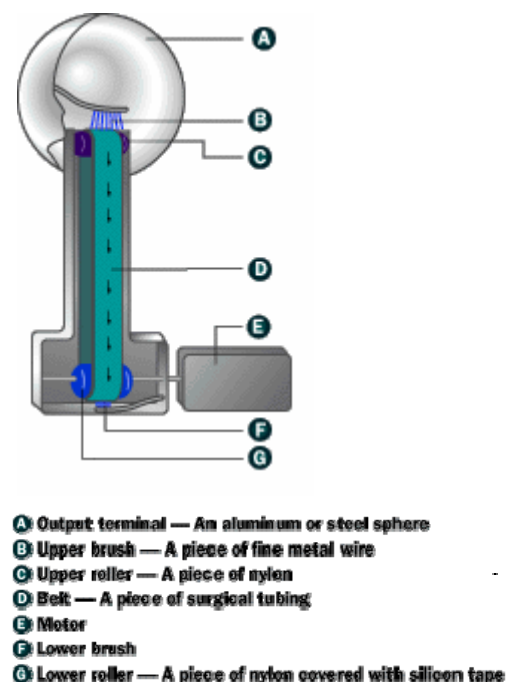
Figure 1: A Van de Graaff Generator and its Components (Zavisa)
