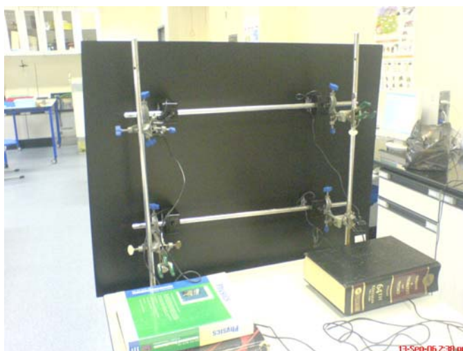
Fig 5 - The finished force plate.
