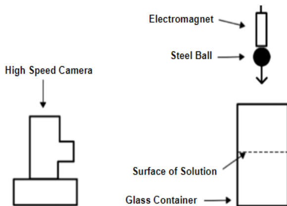
Figure 2. Diagram of the apparatus.
