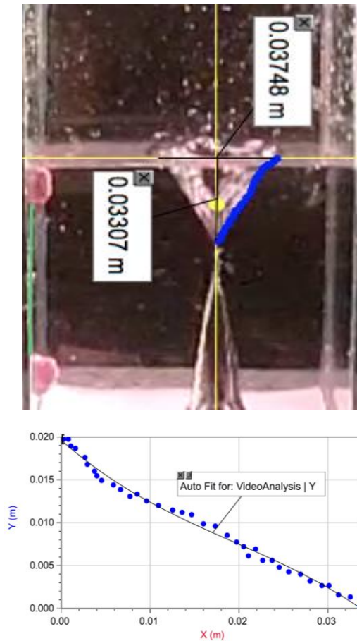
Figure 3. The wall of the cavity is plotted at pinch-off (blue dots). Axes are created, and cavity depth and width are measured. Then, the shape of the cavity is modelled with a function.
