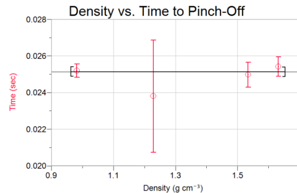
Figure 6. Time between impact and cavity pinch-off is shown here to be independent of density.
