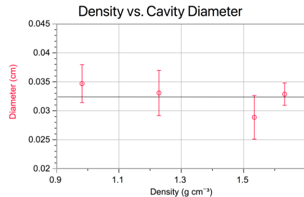
Figure 5. Cavity diameter at pinch-off is independent of density.
