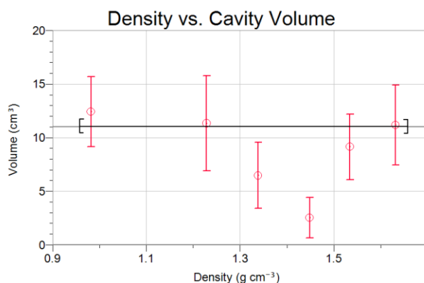
Figure 7. Cavity volume vs density for all six densities tested. The trailing air cylinder did not fully form for densities of 1.34 and 1.45 \text{ g}\cdot\text{cm}^{-3}
