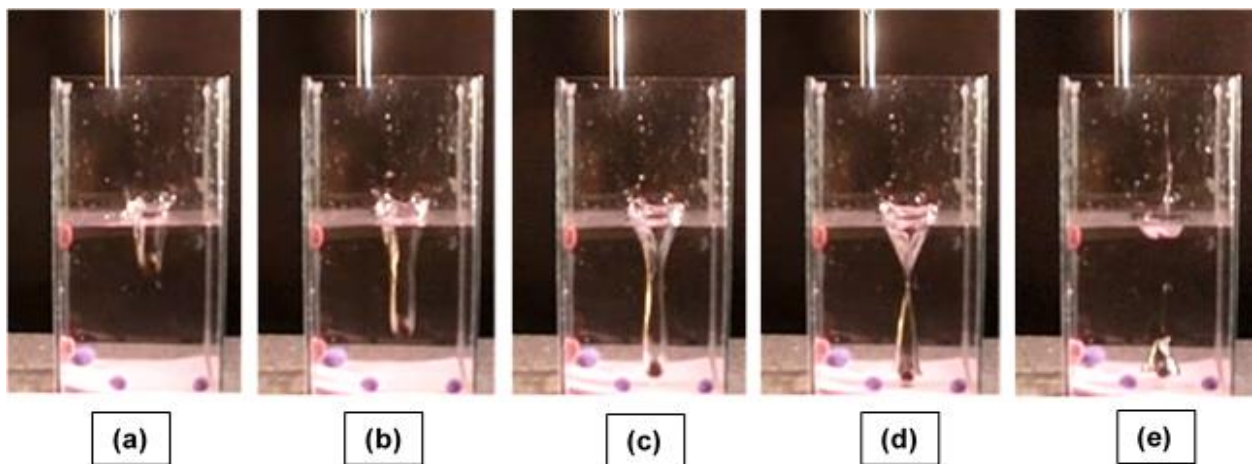
Figure 1. The process of cavity formation and collapse. Example from trial 1 of liquid density 0.98 \text{ g}\cdot\text{cm}^{-3} .
