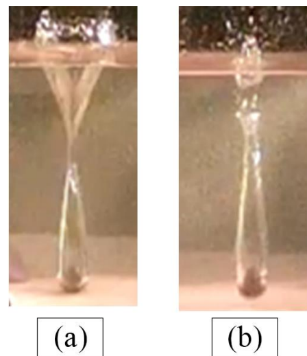
Figure 8. The cavity formation for liquid density 1.63 \text{ g}\cdot\text{cm}^{-3} (a) is clearly different from the cavity formation for 1.45 \text{ g}\cdot\text{cm}^{-3} (b).
